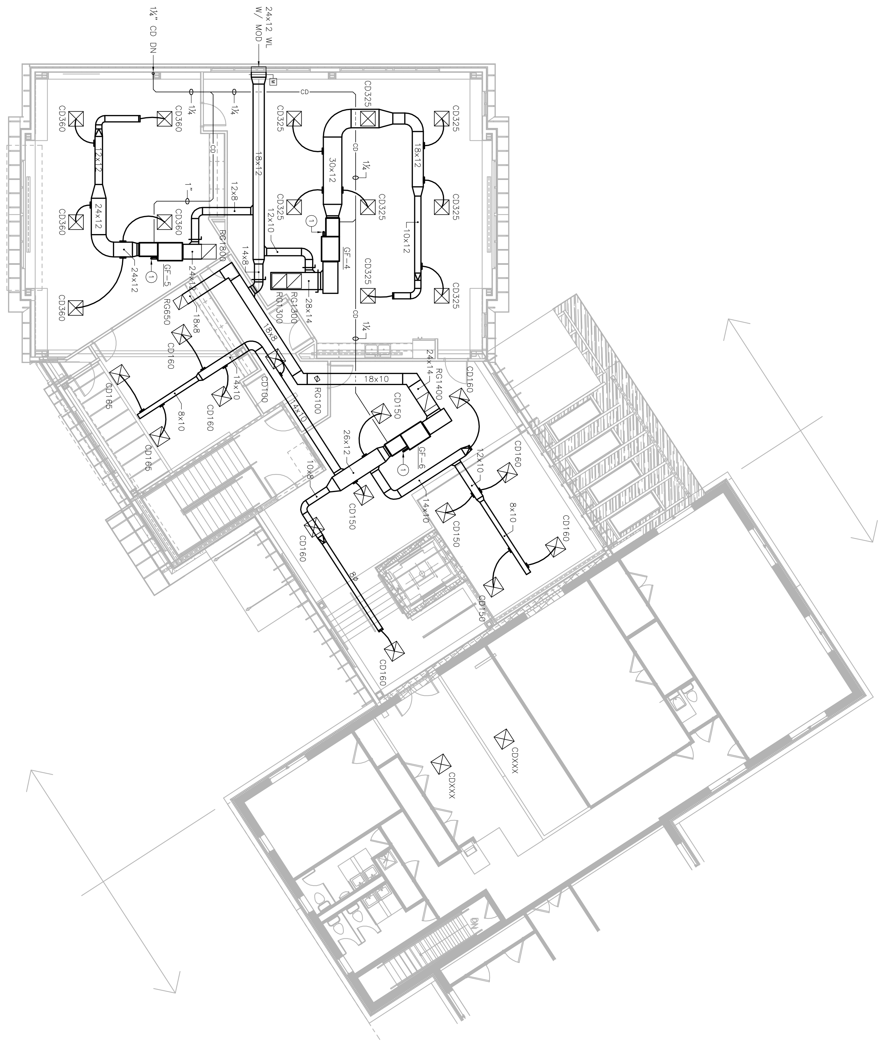
2 UPPER LEVEL FLOOR PLAN - HVAC 1/8" = 1'-0"
