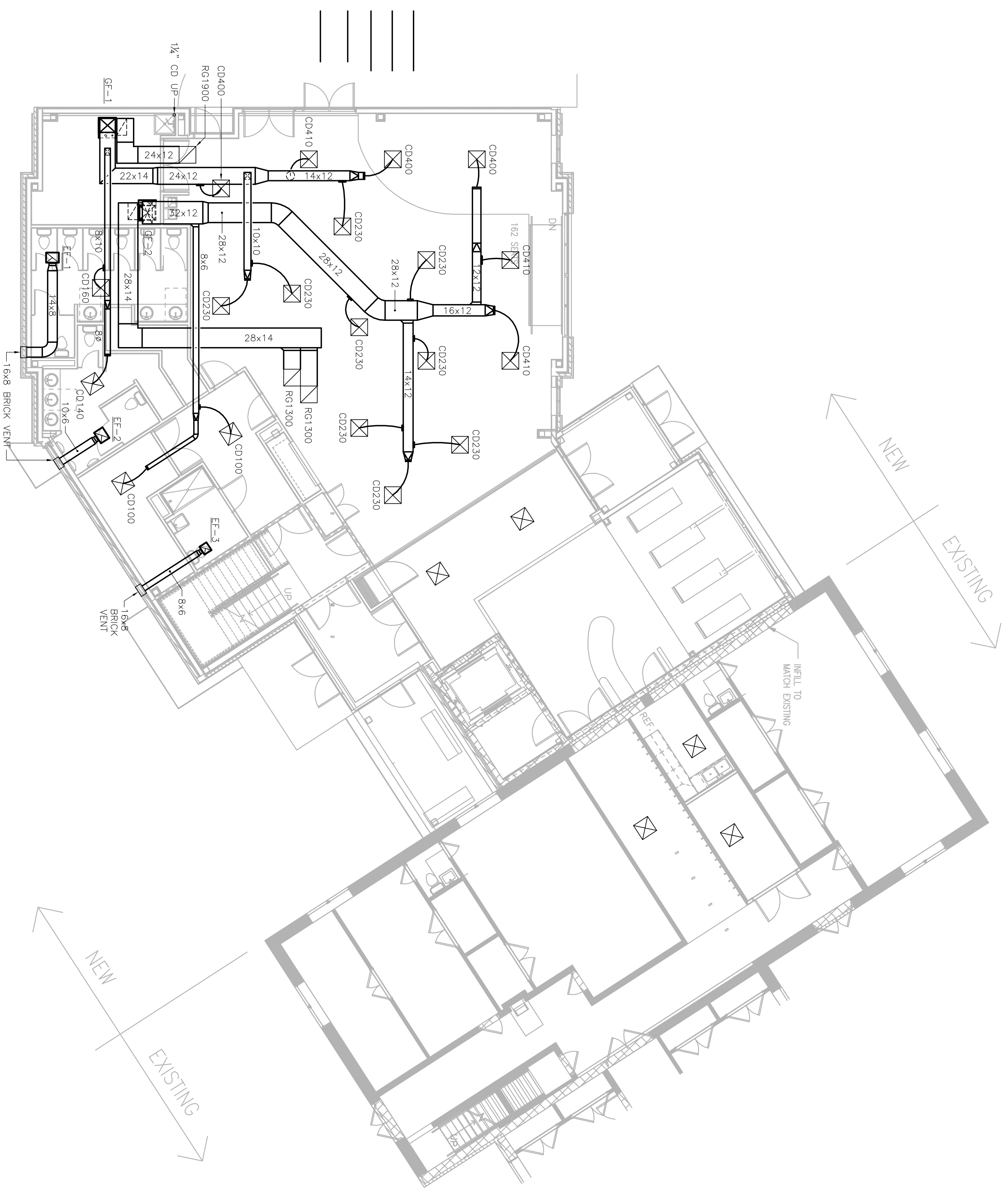
1 LOWER LEVEL FLOOR PLAN - HVAC 1/8" = 1'-0"
