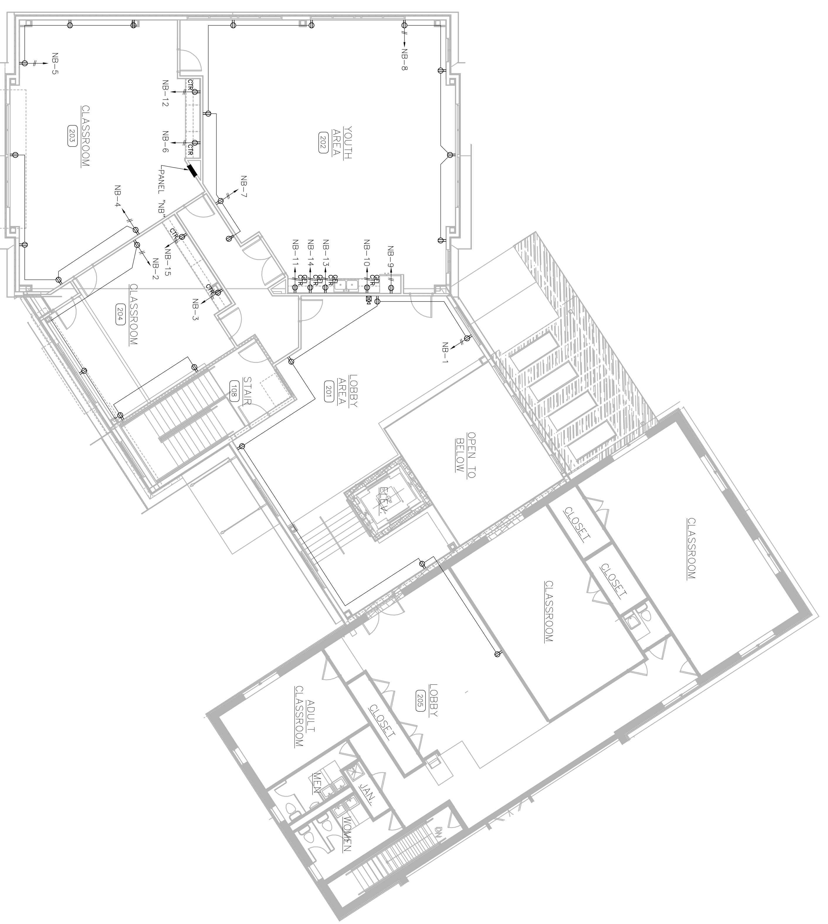
4 UPPER LEVEL FLOOR PLAN - POWER 1/8" = 1'-0"
